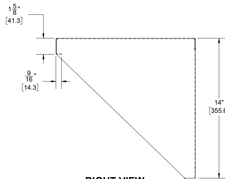
RIGHT VIEW
